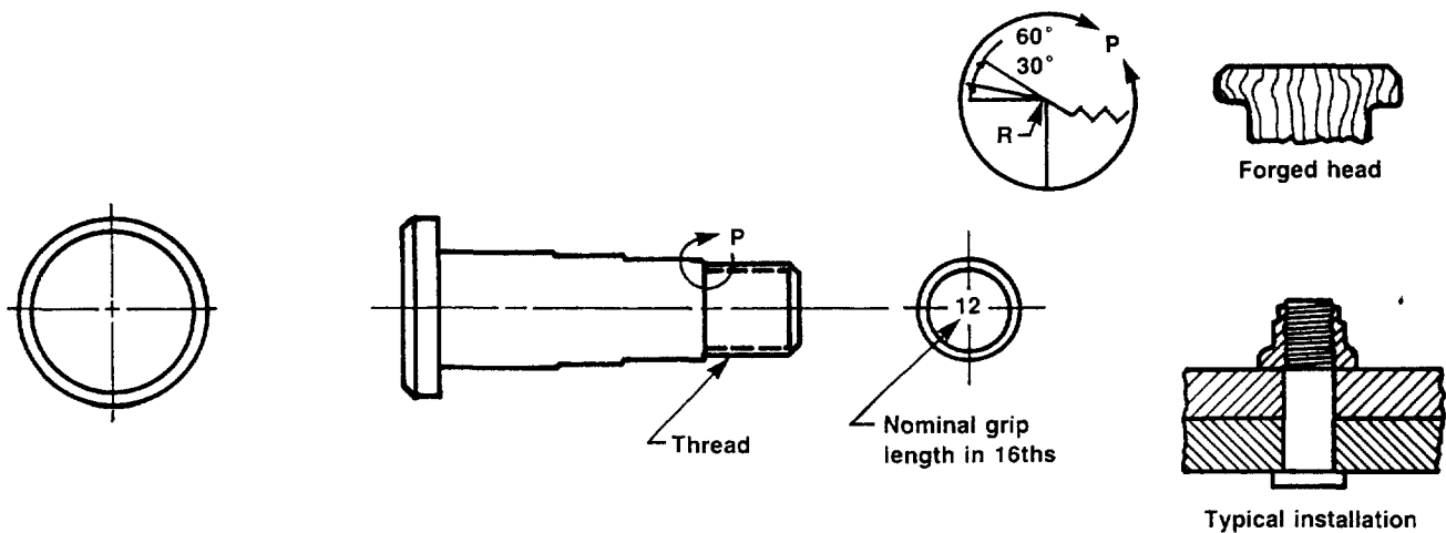
Figure 51.—Taper-Lok installation.
